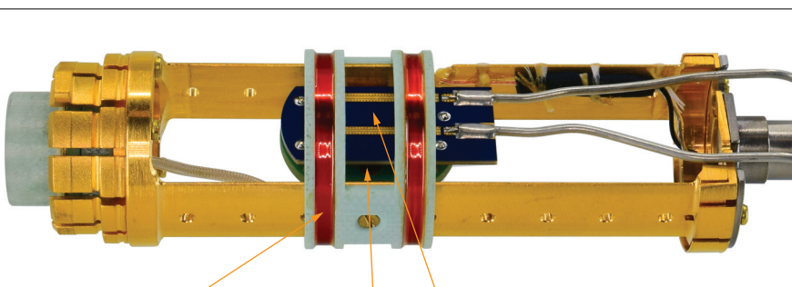
Helmholtz coils for field modulation
