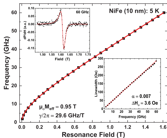
In-plane CryoFMR (2-60 GHz) of a 10 nm thick Permalloy film
