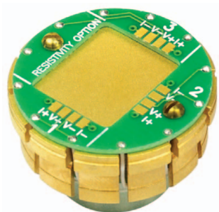
Resistivity Puck (QD part number: 8084-109)
