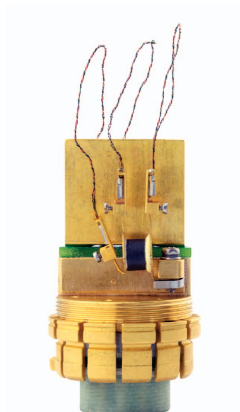
TTO Puck with Disk-Shaped Sample Installed
