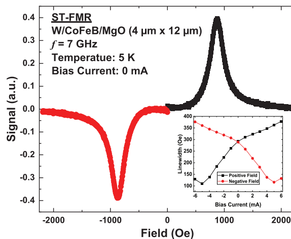
Cryo ST-FMR of a patterned W/CoFeB device
