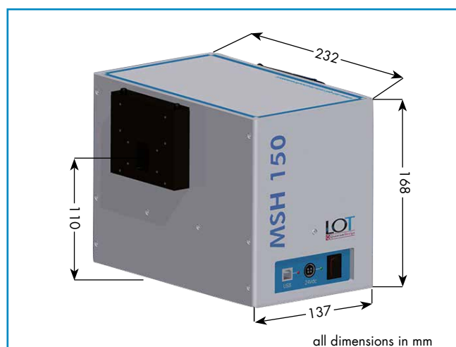
Layout MSH-150F
