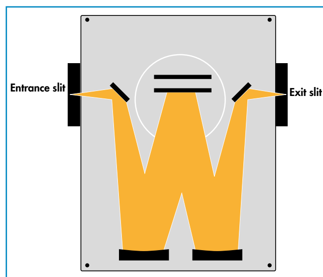
Optical configuration: MSH-150F monochromator
